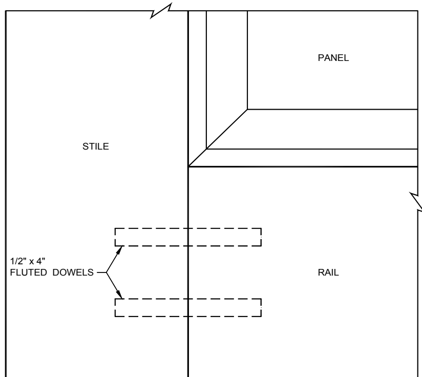
CORNER ELEVATION
