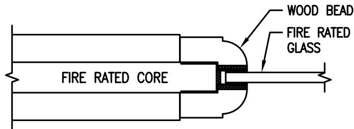
STANDARD PROFILE – WOOD BEAD
